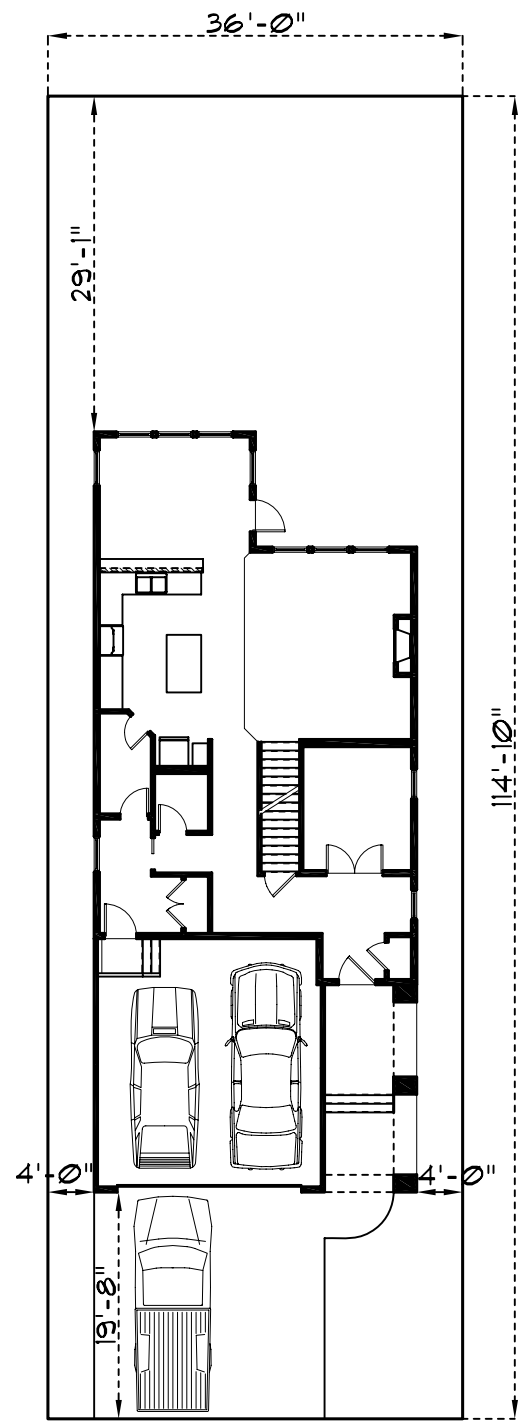
LARGE CITY LOT w/2500 sq. ft. HOUSE
