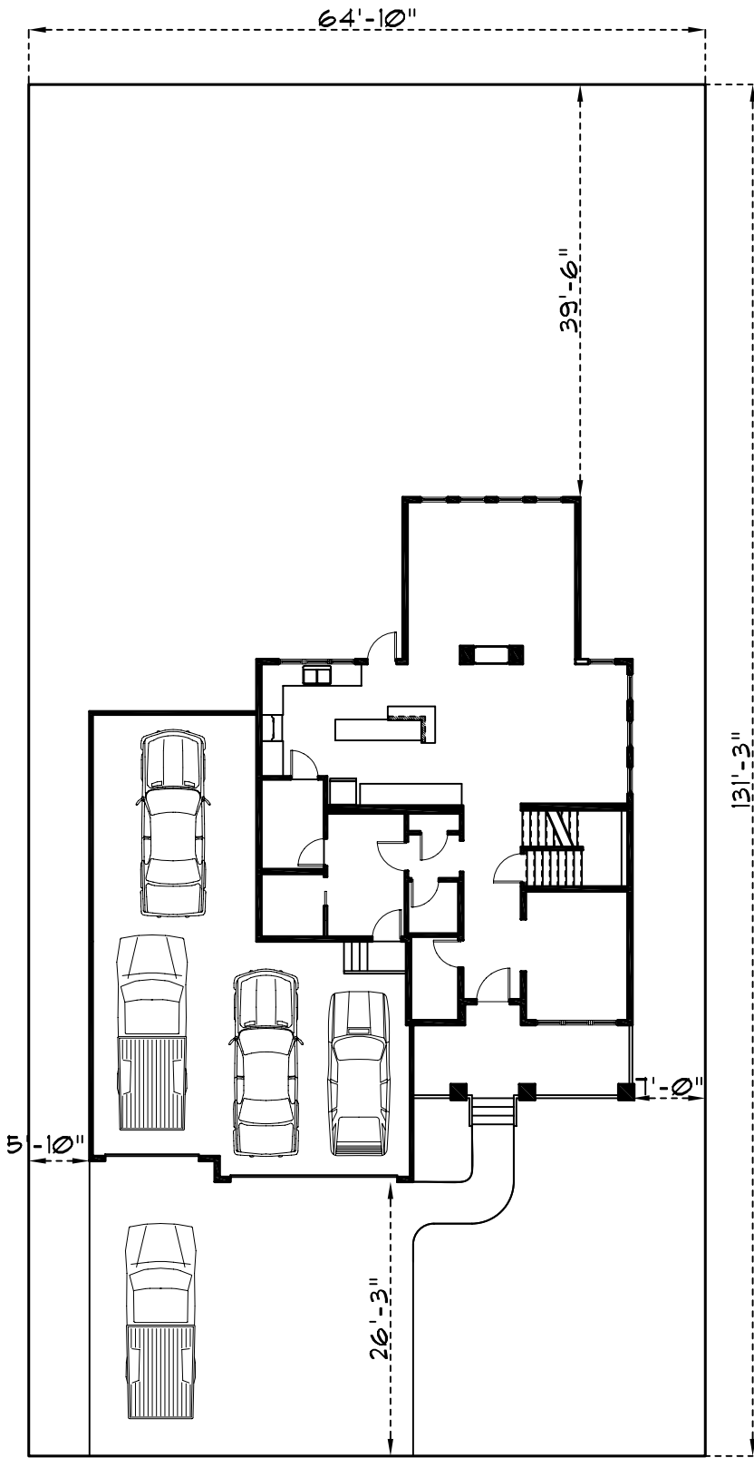
BOULDER CREEK LOT w/2500 sq. ft. HOUSE
