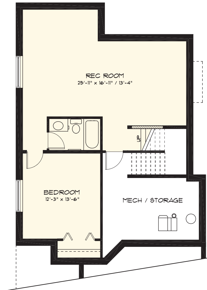
BASEMENT DEVELOPMENT OPTION TOTAL AREA - 676 Sq. Ft.
