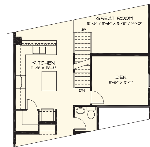
DEVELOPED STAIR OPTION
