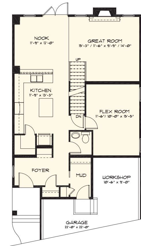
FLEX ROOM OPTION ADDS 58 Sq. Ft. REVISED MAIN FLOOR AREA - 1011 Sq. Ft.
