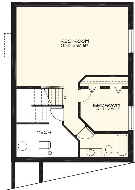
BASEMENT DEVELOPMENT OPTION TOTAL AREA - 594 Sq. Ft.
