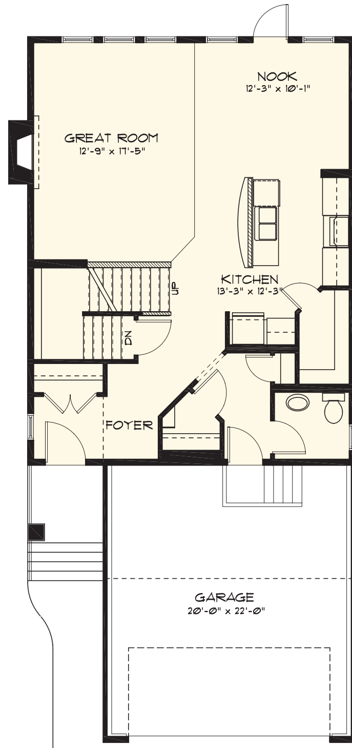
MAIN FLOOR STOCKPLAN 884 Sq. Ft.
