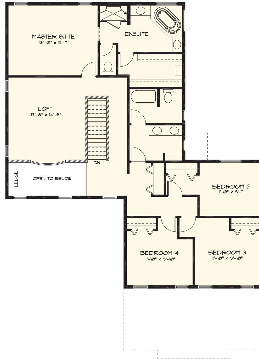
UPPER FLOOR STOCK PLAN 1551 Sq. Ft.
