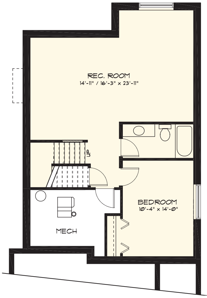
BASEMENT DEVELOPMENT OPTION TOTAL AREA - 626 Sq. Ft.
