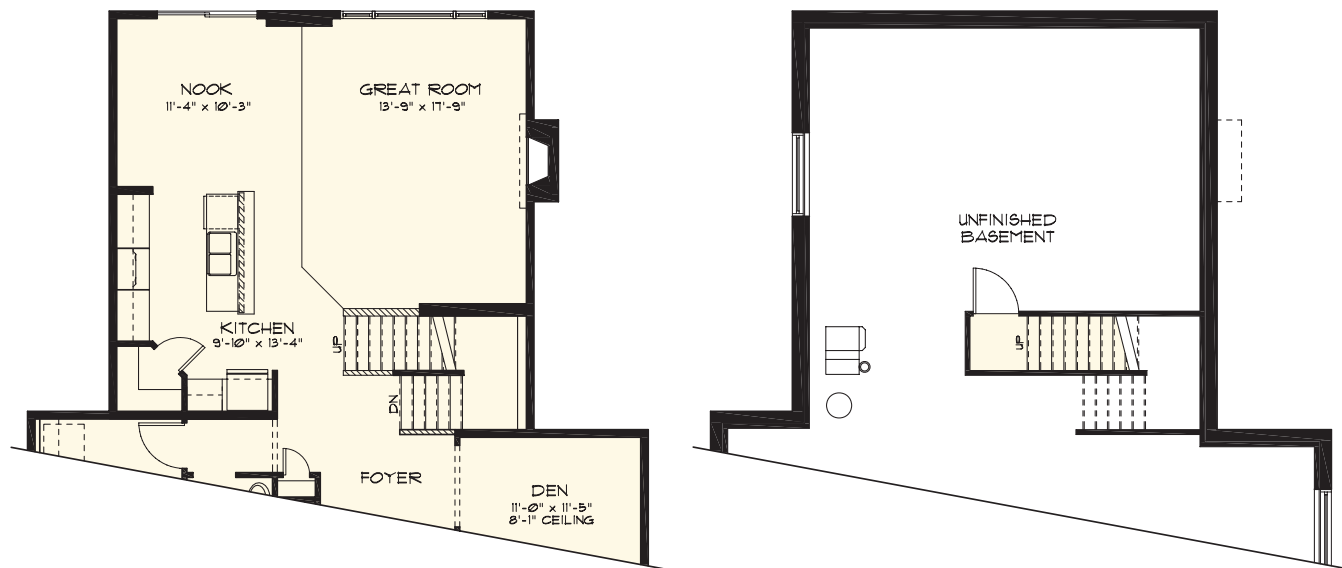
DEVELOPED STAIR OPTION
