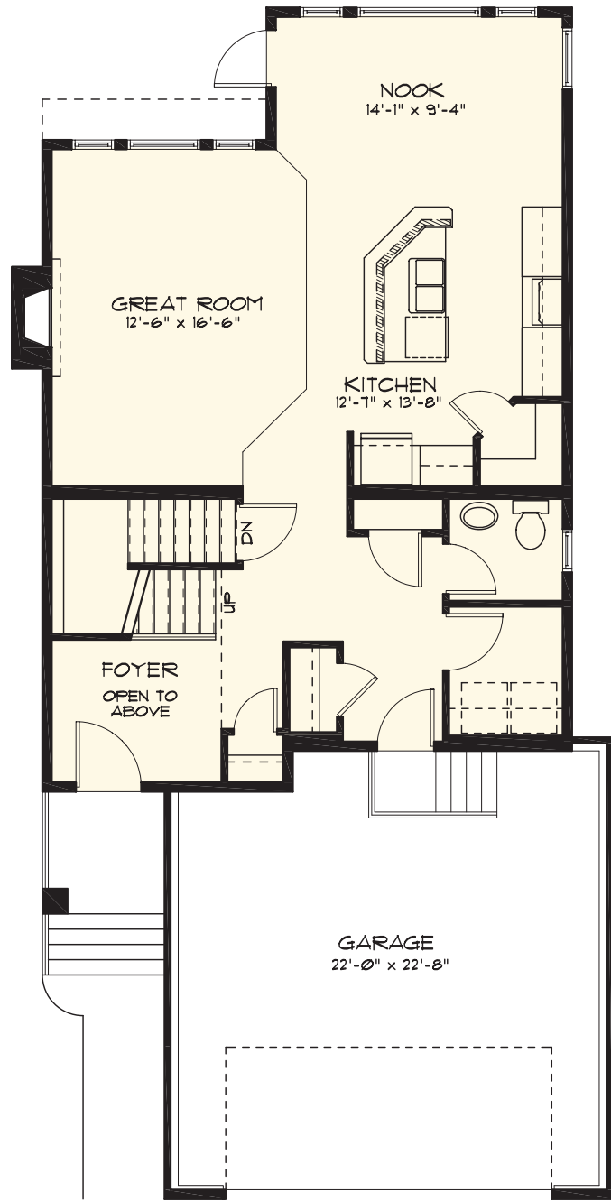
MAIN FLOOR STOCKPLAN 902 Sq. Ft.
