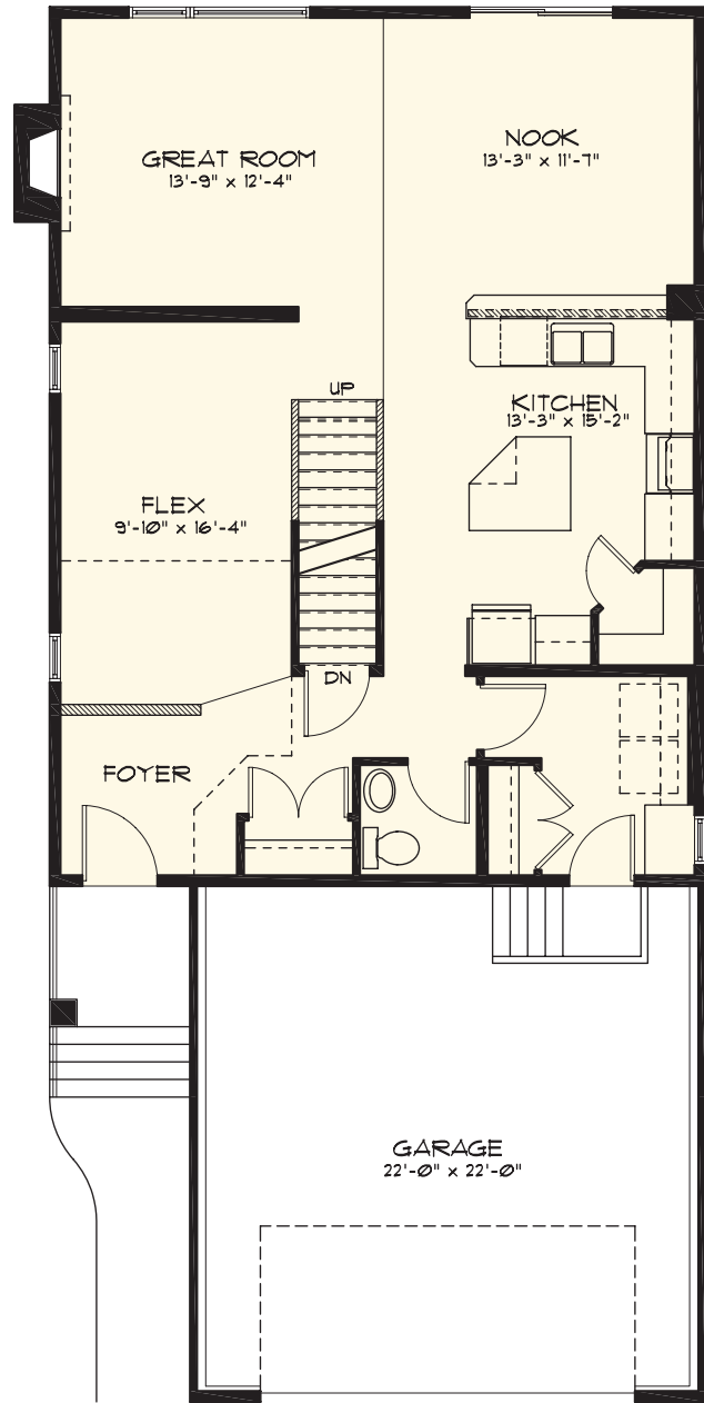
MAIN FLOOR STOCKPLAN 1050 Sq. Ft.
