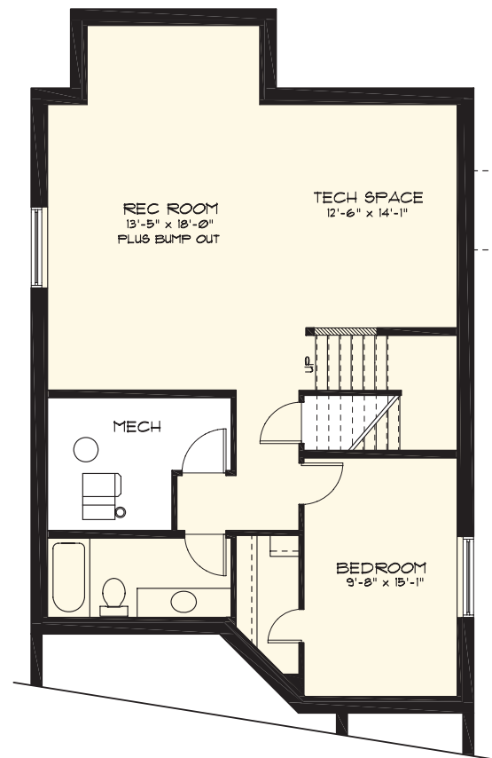
BASEMENT DEVELOPMENT OPTION TOTAL AREA - 781 Sq. Ft.
