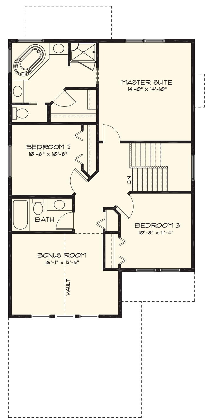
3 BEDROOM & BONUS ROOM OPTION ADDS 21 Sq. Ft. TOTAL UPPER FLOOR 1099 Sq. Ft.
