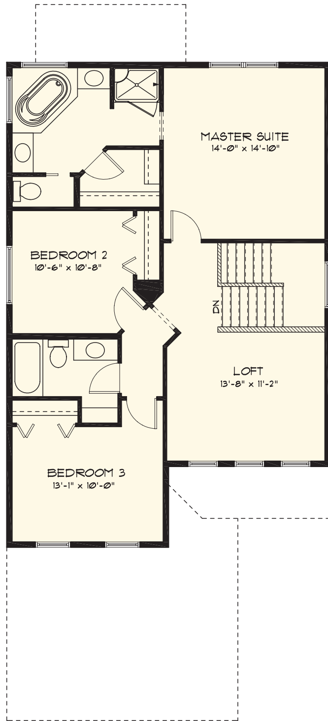
UPPER FLOOR STOCKPLAN 1078 Sq. Ft.
