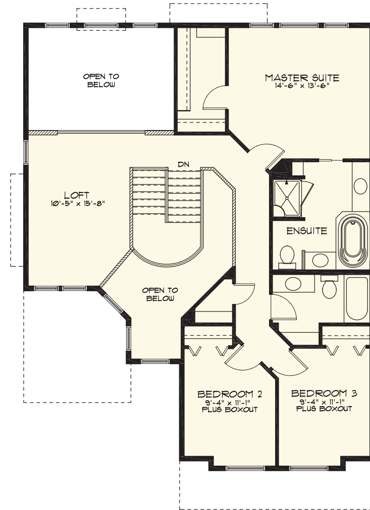
UPPER FLOOR STOCK PLAN 1135 Sq. Ft.
