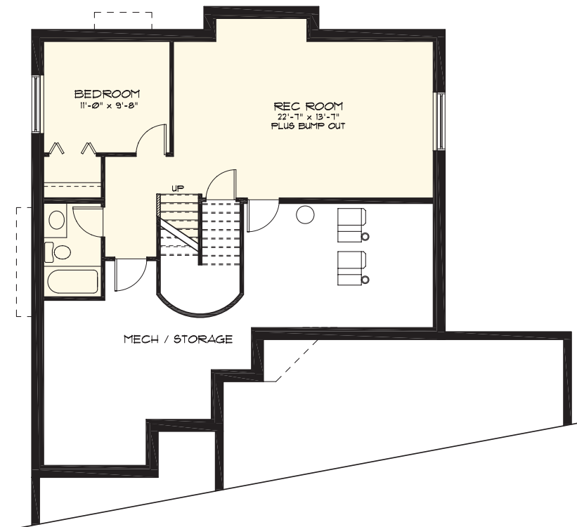
BASEMENT DEVELOPMENT OPTION TOTAL AREA - 548 Sq. Ft.
