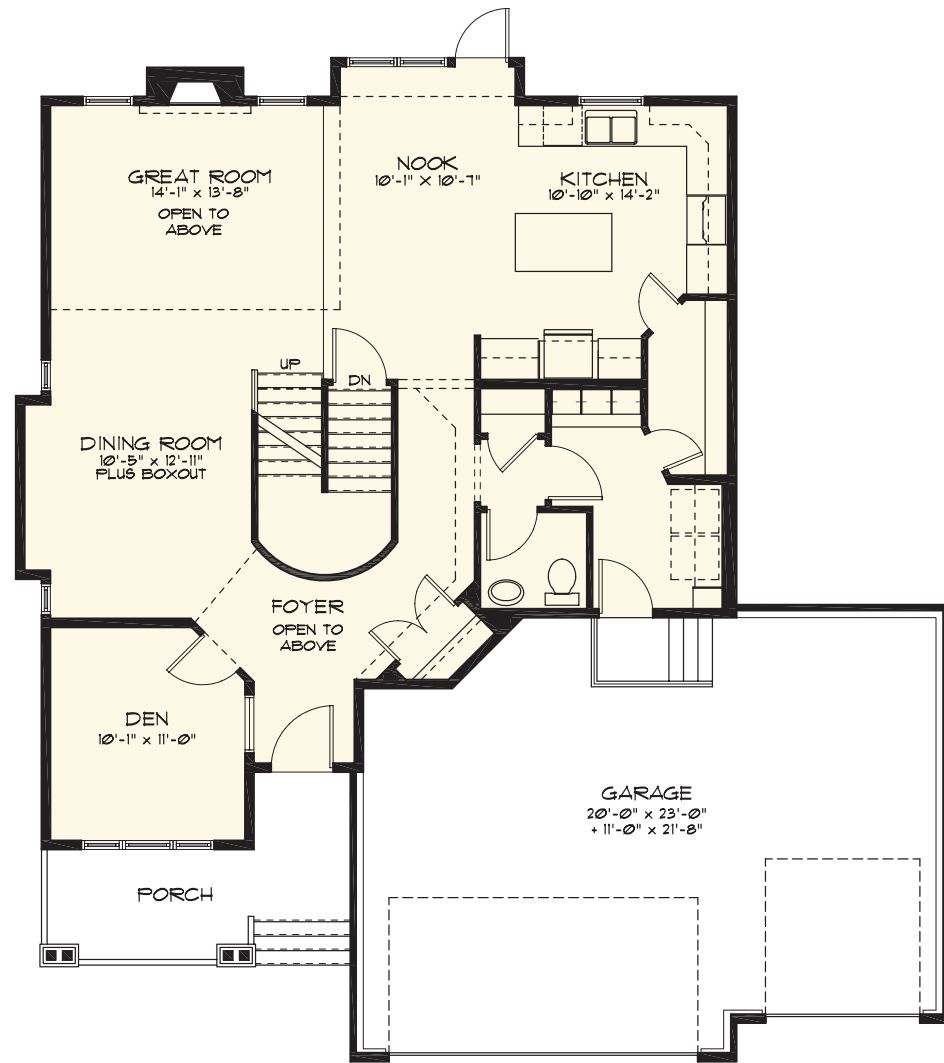
MAIN FLOOR STOCK PLAN 1206 Sq. Ft.
