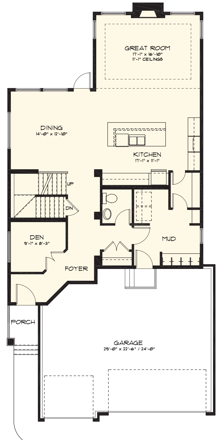
TRIPLE CAR GARAGE OPTION ADDS 15 Sq. Ft. TO MAIN FLOOR TOTAL MAIN FLOOR - 1235 Sq. Ft.
