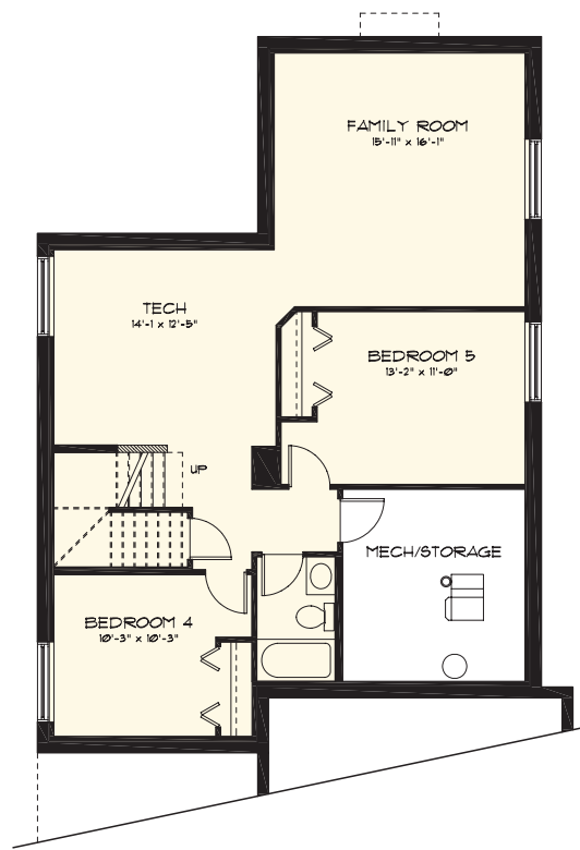
BASEMENT DEVELOPMENT 2 BEDROOM OPTION TOTAL AREA - 843 Sq. Ft.
