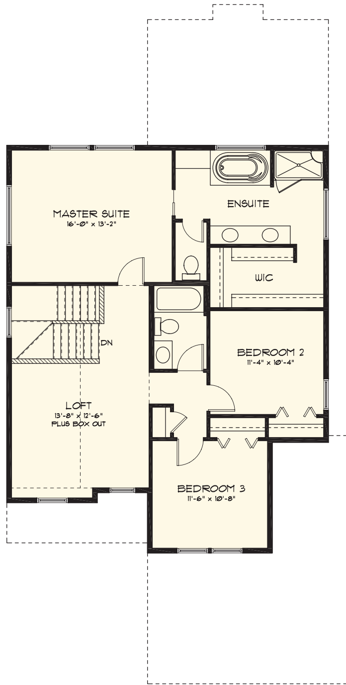
UPPER FLOOR 1160 Sq. Ft.
