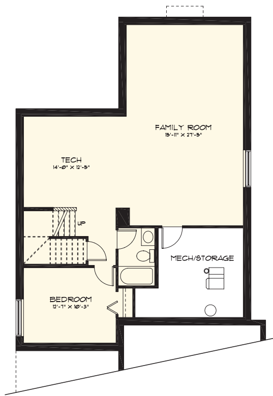
BASEMENT DEVELOPMENT OPTION TOTAL AREA - 835 Sq. Ft.
