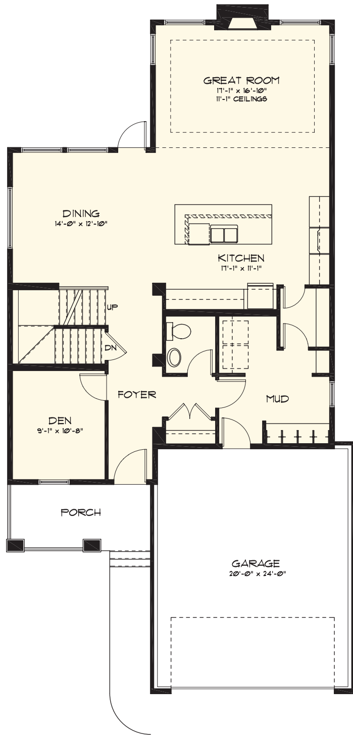
MAIN FLOOR 1220 Sq. Ft.
